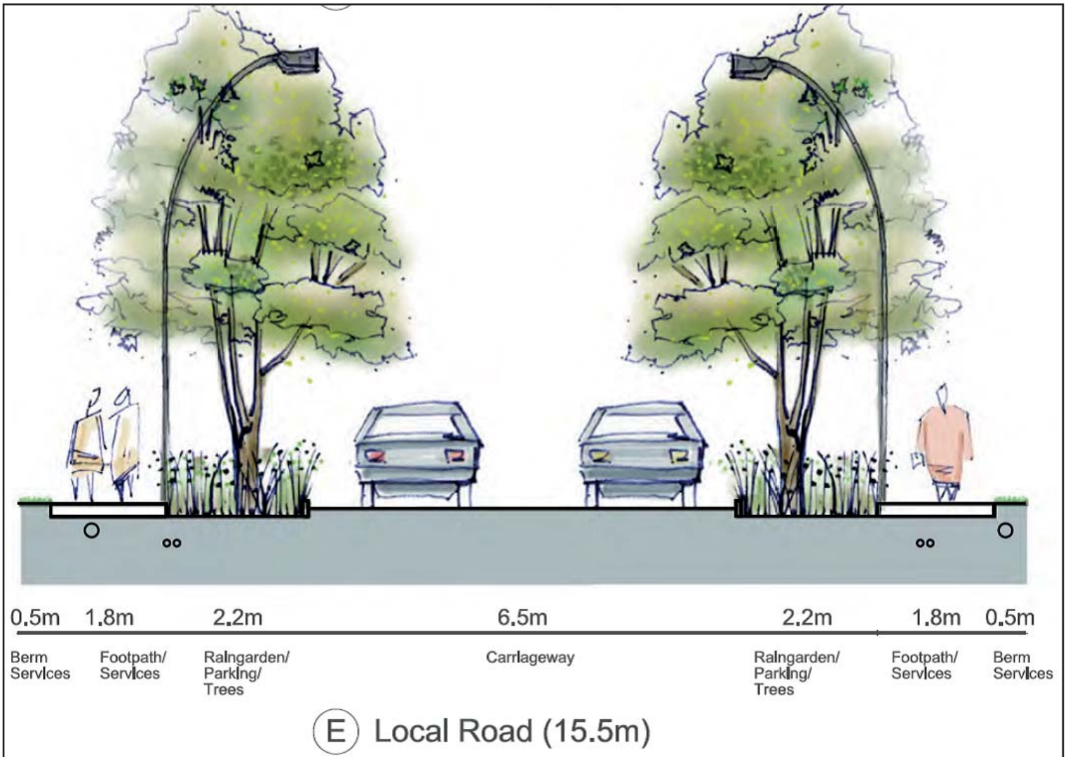
Figure 8: Type E road
